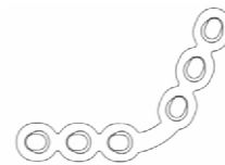
Kieferwinkelplatte 6-Loch Mandibular angle plate 6-hole 13.031.06
